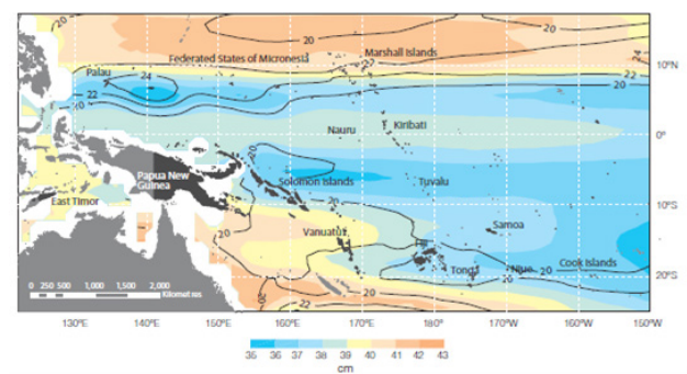
Figure 6. Sea-level projections (in cm) for the A1B (medium) emissions scenario in the PCCSP region for 2061–2100 relative to 1981–2000
