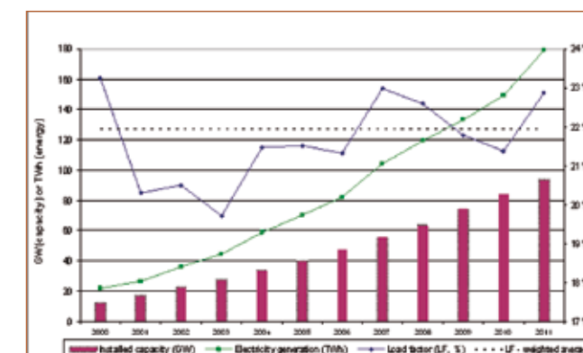
Figure 2: Wind energy generation, installed capacity and load factors. The whole wind farm park in Europe has had a clear increasing capacity over the last ten years.
