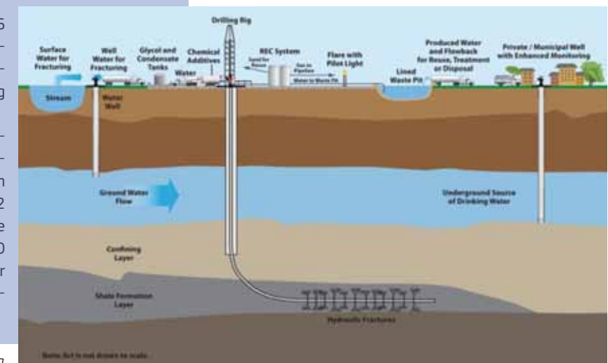
Hydraulic fracturing.
