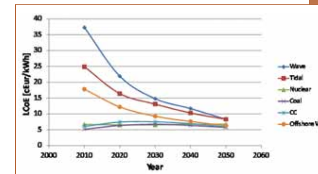
Expected evolution of the energy costs for different sources until 2050. LCoE = levelised cost of energy (the price at which electricity must be generated from a specific source to break even over the lifetime of the project).
